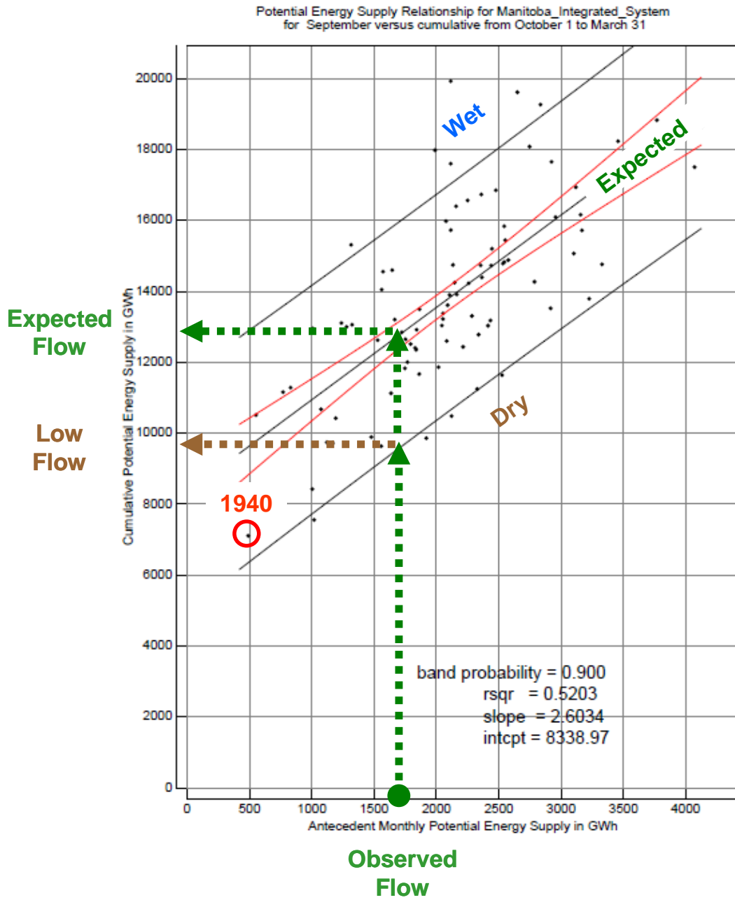
Figure 2. Antecedent regression relationship of potential energy from inflows for the antecedent month of September.
