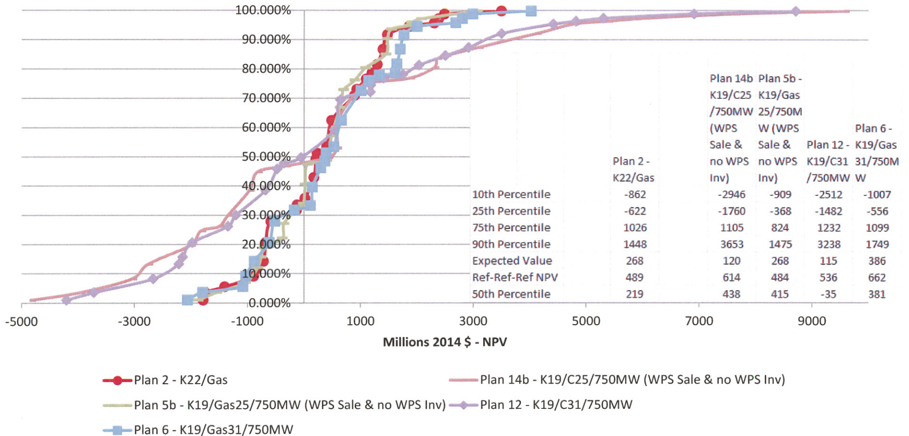
S Curves: No Intertie vs. 750 MW Intertie (No Inv) - Revised
