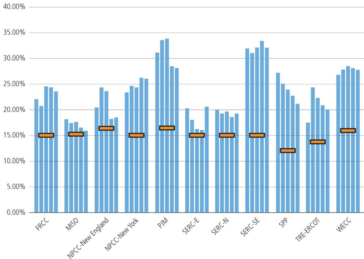
Figure 4.2. Five-Year Average Reserve Margins across Different Regions (2018–2022) 231
