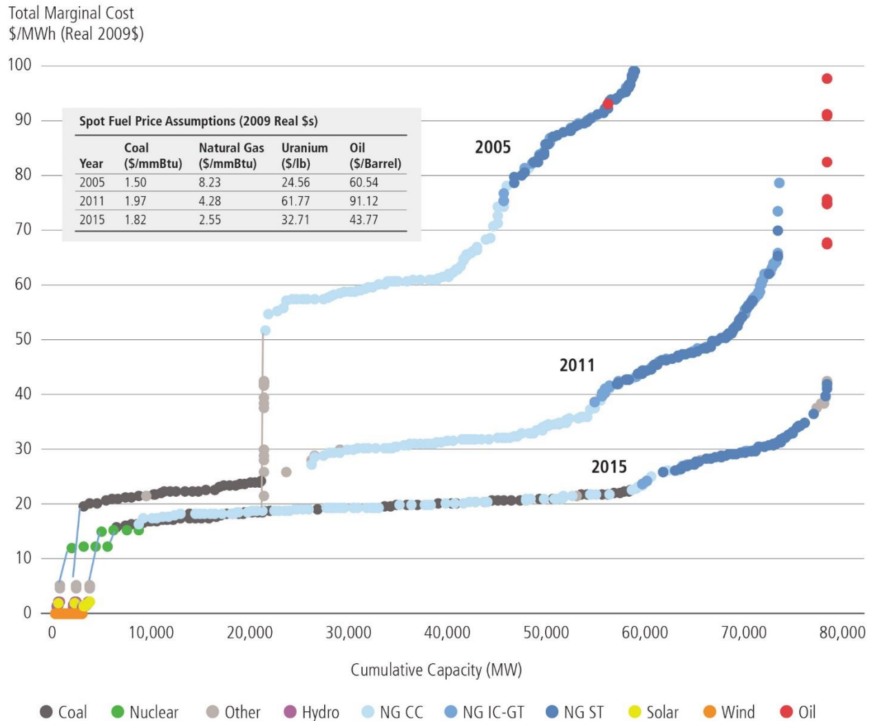
Figure 5.5. Simulated ERCOT Dispatch Curves xxx
